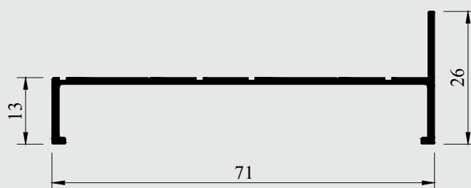
Marco lateral
